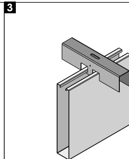
U-Carrier
